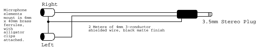
Microphone Assembly
